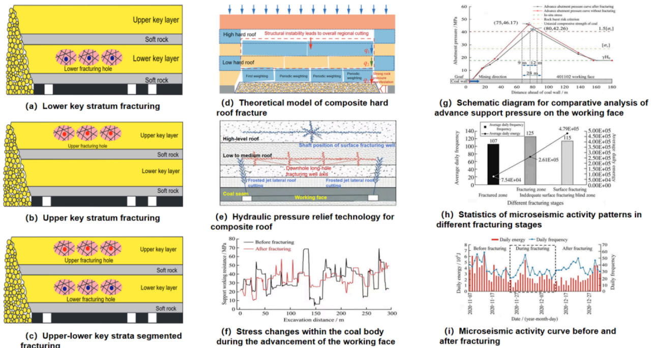
Figure 3. Comparison of overburden structure regulation and rock burst prevention effects under different fracturing modes (a, b, c modified from reference [2], d [22], e [33], f [34], g [28], h [29], i [34])
