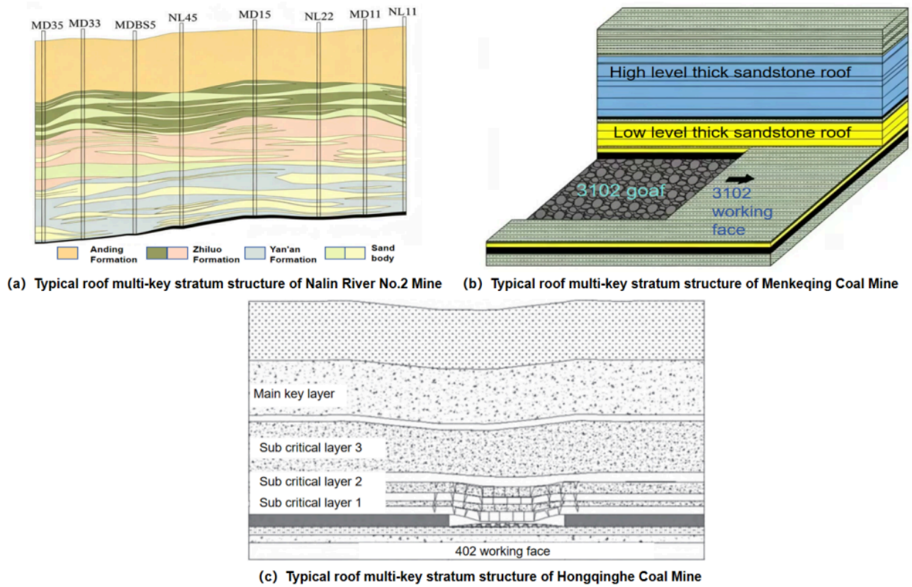
Figure 1. Examples of typical multi-key-stratum roof structures in multiple locations in the Meng-Shaan mining area (a modified from reference [4], b [8], c [9])
