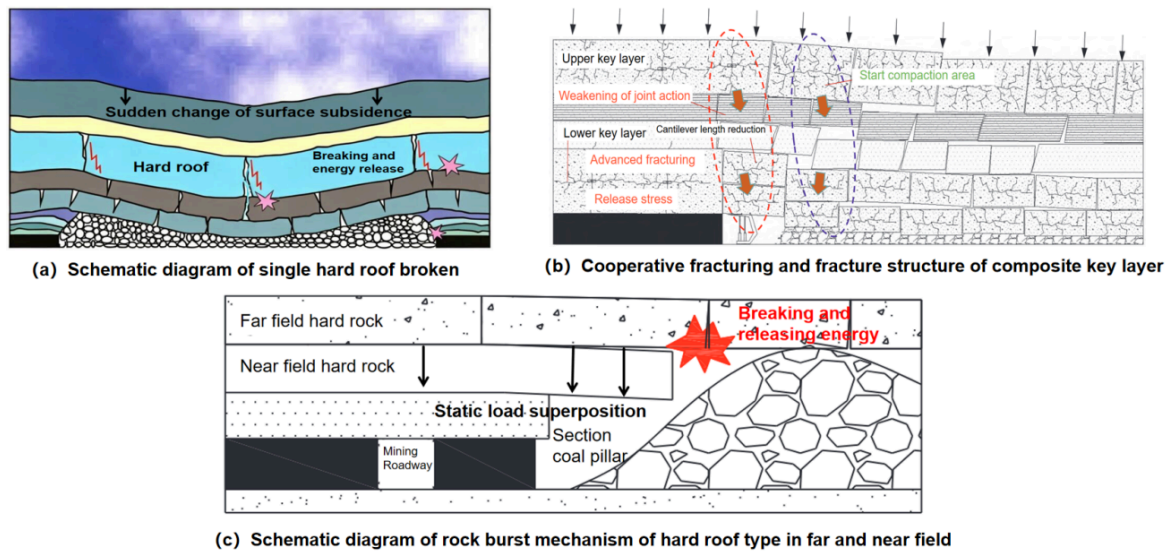
Figure 2. Schematic diagram of disaster-inducing mechanism of different types of hard roof fracture (a modified from reference [26], b [2], c modified from reference [1])
