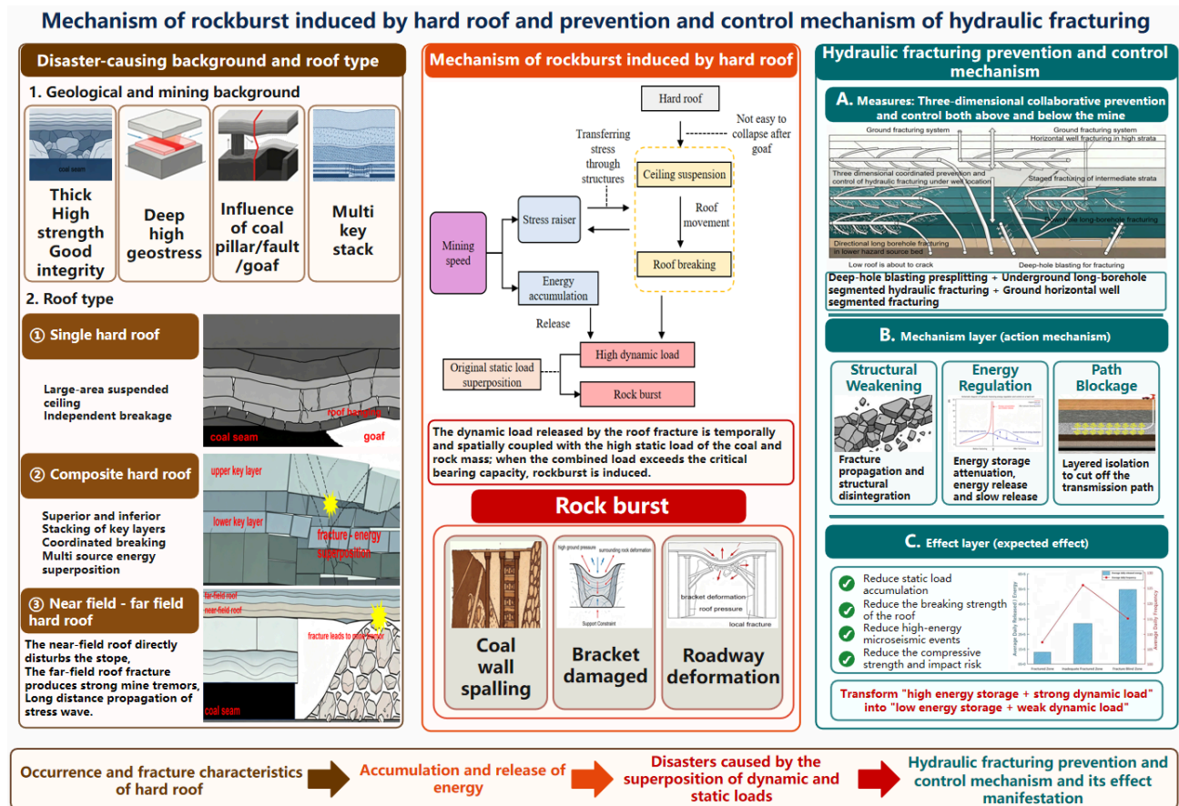
Figure 5. Discussion on mechanism of rock burst induced by hard roof and hydraulic fracturing prevention and control technology
