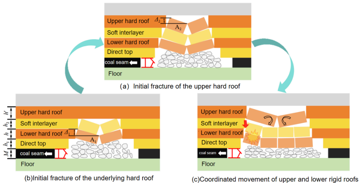
Figure 4. Three-stage evolution of composite hard roof fracture and migration under mining action [39]
