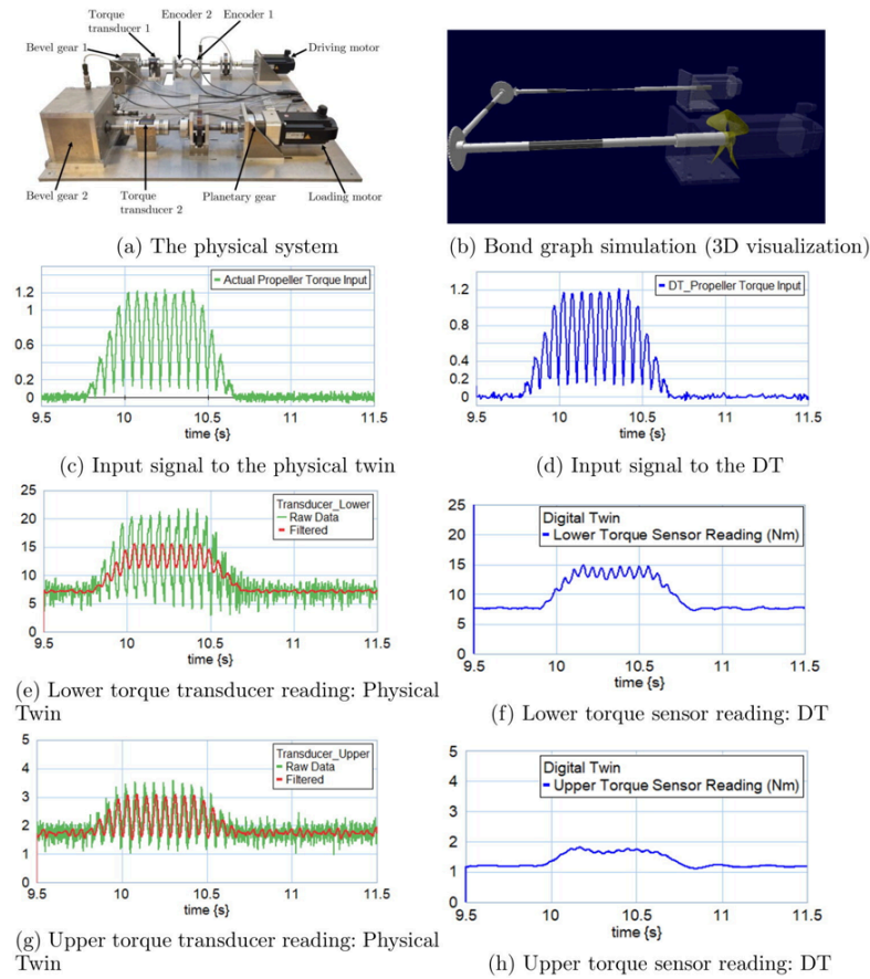
Figure 5. Comparison of actual torque response and digital twin simulation results under propeller-ice interaction conditions [6]
