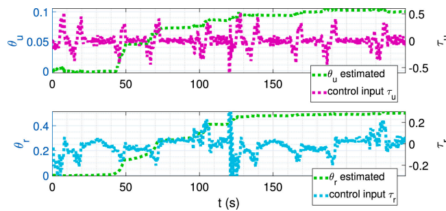
Figure 4. Estimated results of propeller fault parameters under fault status [5]
