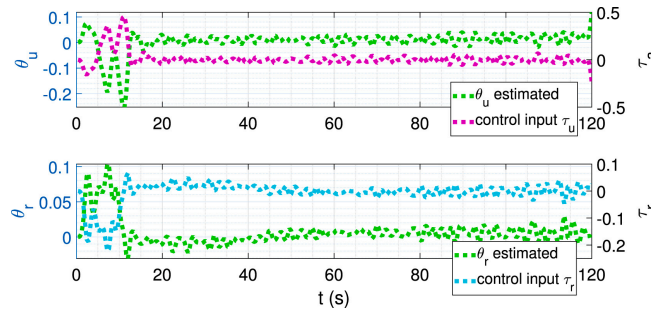
Figure 3. Estimated results of propeller fault parameters under normal operating status [5]
