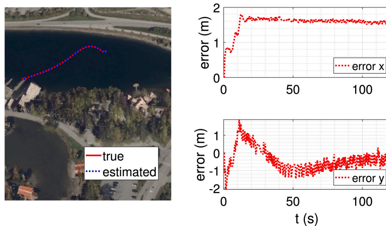
Figure 1. Comparison between the actual vessel trajectory and digital twin estimates under normal operation [5]
