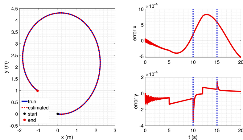
Figure 2. Comparison between the actual vessel trajectory and digital twin estimates under propeller fault conditions [5]
