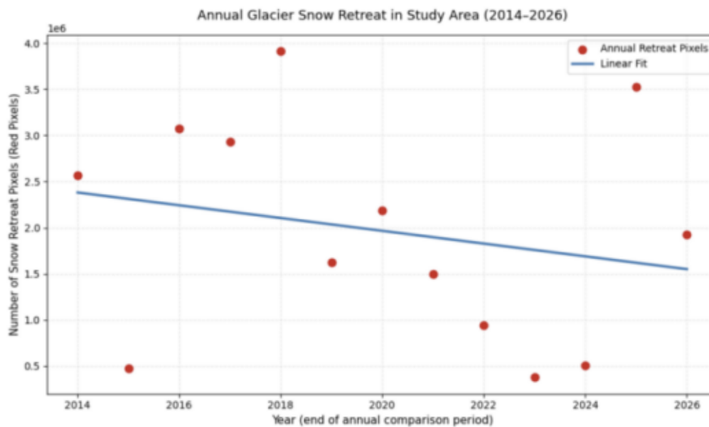
Figure 4. Plot of annual net snow retreat (red pixel count) in the study area over the time period from August 2013 to August 2026, with the blue line showing the linear line of best fit
