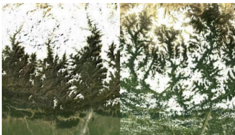
Figure 2. True-color Landsat 8 satellite images of the study area, February 2022 (left) and August 2022 (right)
