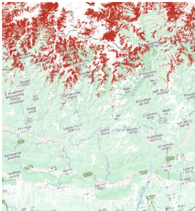
Figure 3. Seasonal snow cover change map derived by subtracting the February 2022 NDSI snow map from the August 2022 NDSI snow map and removing false colors
