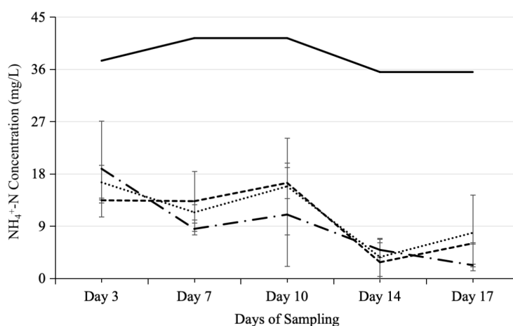
Figure 3. NH 4 + -N concentration over 17 days (— · Typha orientalis , ····· Acorus calamus , - - - Phragmites communia , — Influent)
