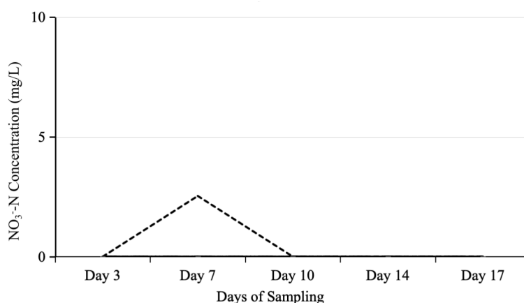
Figure 2. NO 3 - concentration over 17 days (— · Typha orientalis , ····· Acorus calamus , - - - Phragmites communia , — Influent)
