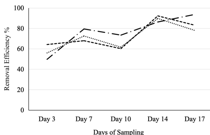
Figure 1. N removal efficiency over 17 days (— · Typha orientalis , ····· Acorus calamus , - - - Phragmites communia , — Influent)
