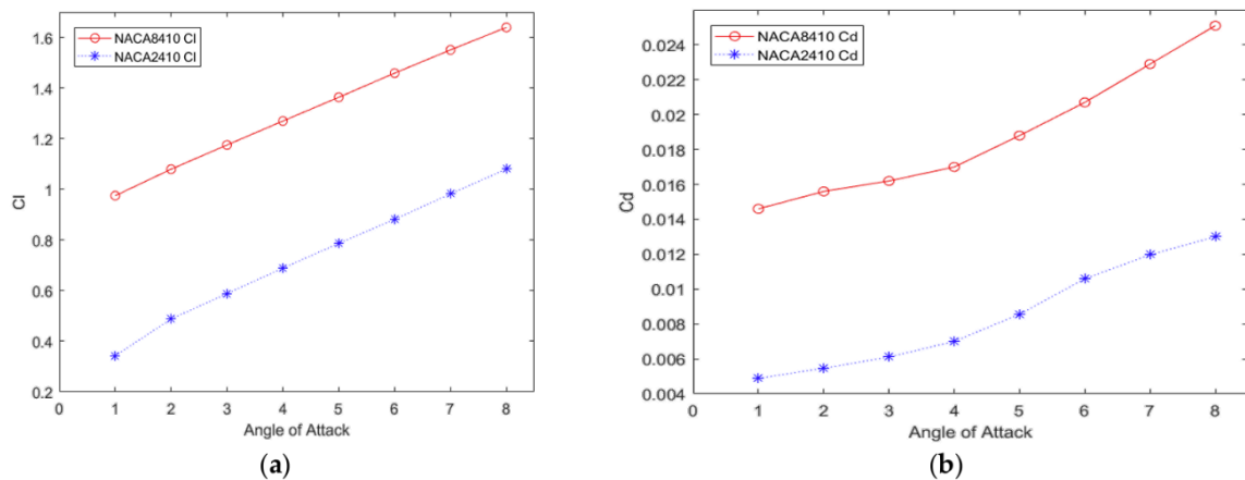
Figure 2. NACA2410 and NACA8410 with changing AoA [3]
