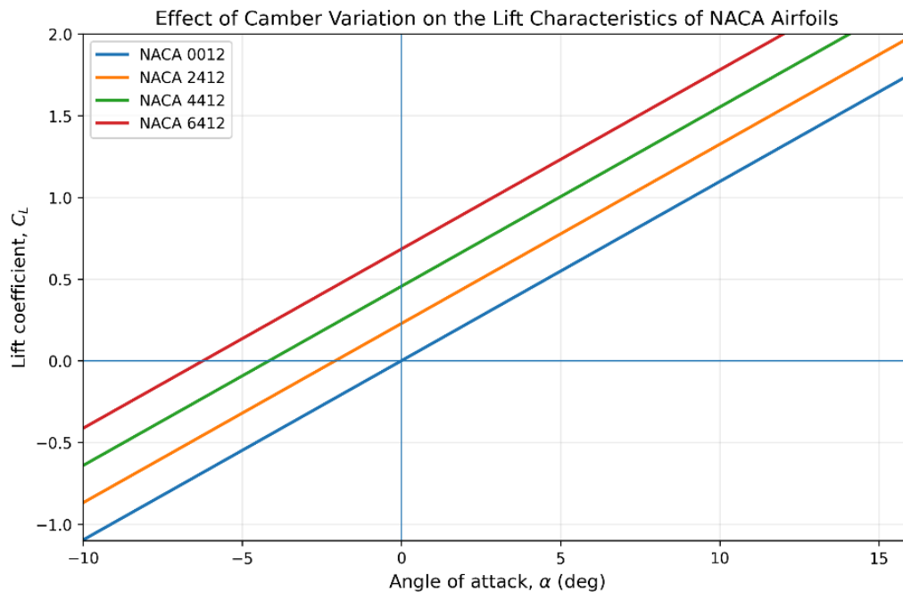
Figure 1. Theoretical influence of camber change on the lift behavior of NACA four-digit wing sections
