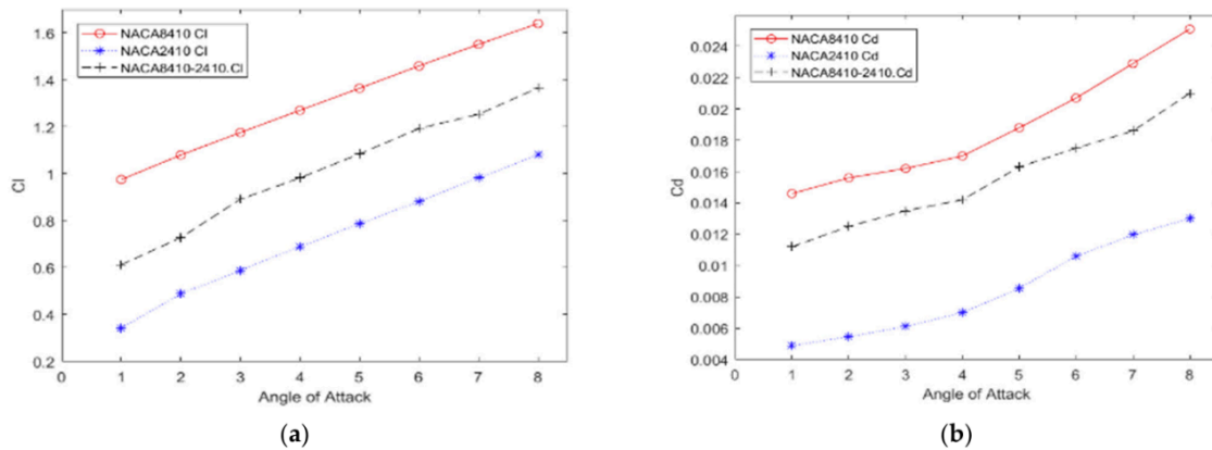
Figure 3. (a) C_L , (b) C_D of NACA2410, NACA8410, and NACA2410 to NACA8410 transition with respect to AoA [3]
