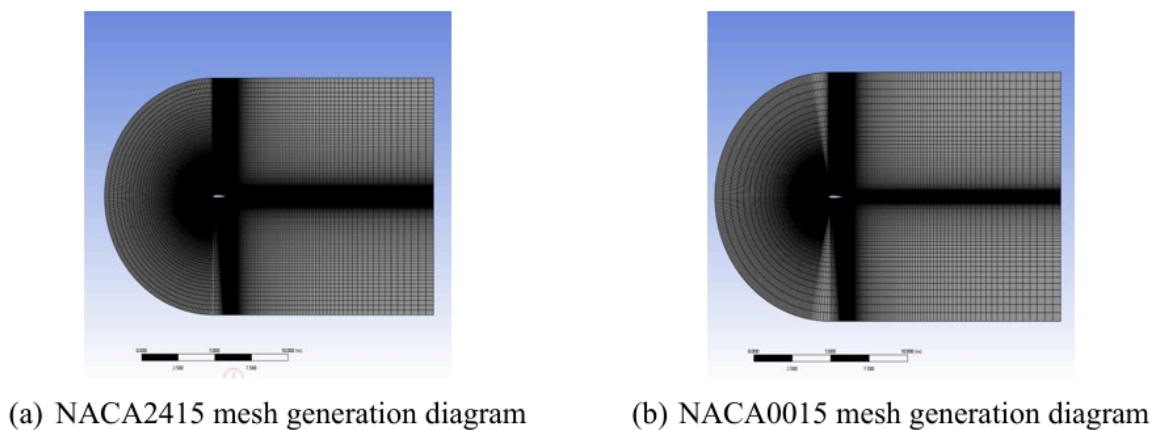
Figure 3. Mesh generation diagrams for NACA2415 and NACA0015 profiles
