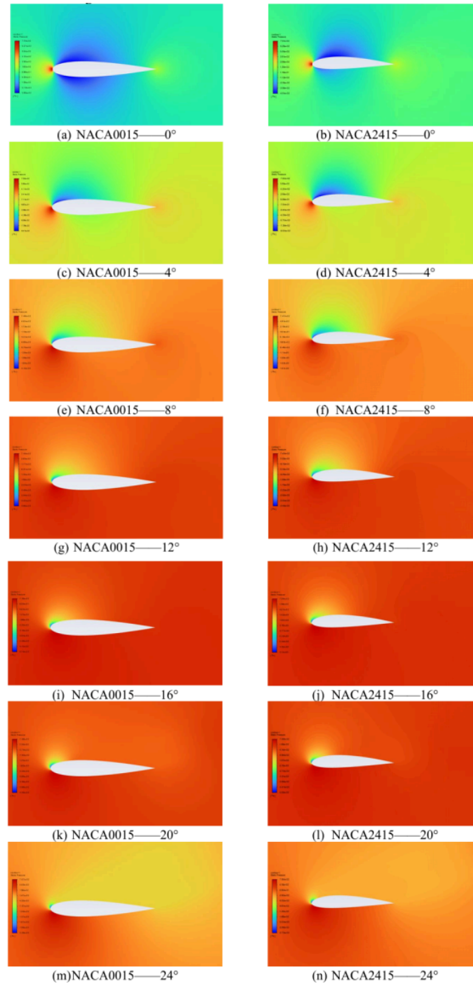
Figure 6. Comparison of pressure contour plots for NACA0015 and NACA2415 at different angles of attack
