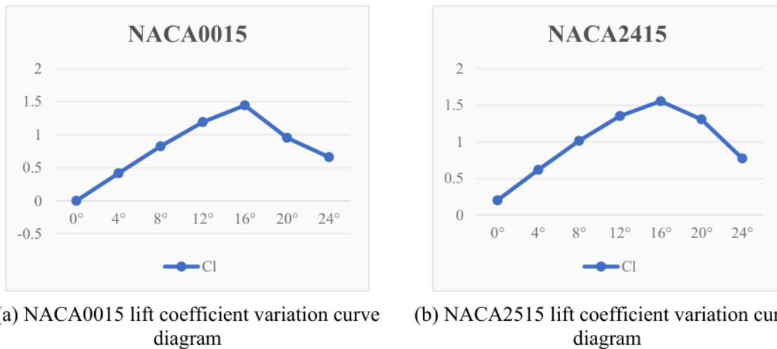
Figure 4. Comparison of lift coefficients for NACA0015 and NACA2425 at different angles of attack
