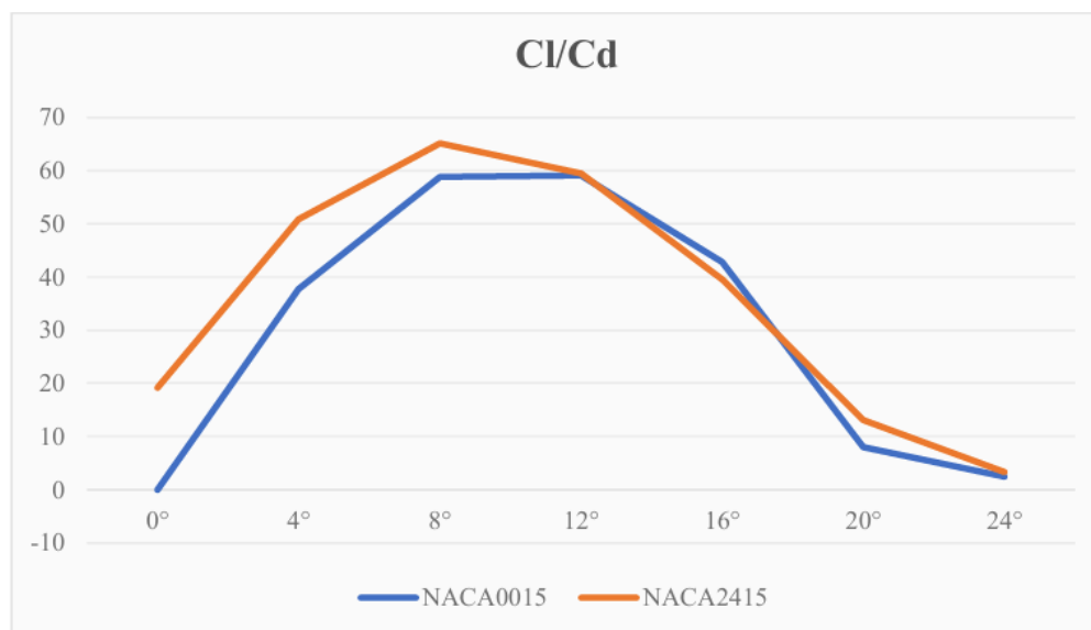
Figure 7. Lift-to-drag ratio of NACA0015 and NACA2415 at various angles of attack
