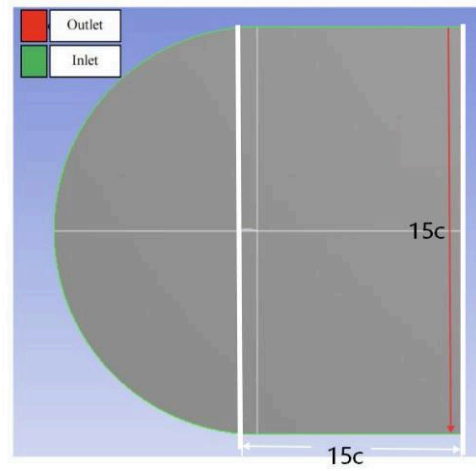
Figure 2. Computational domain of airfoil numerical simulation
