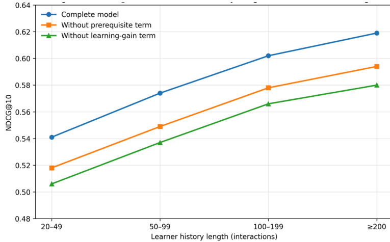
Figure 1. NDCG@10 across learner-history lengths under ablation settings
