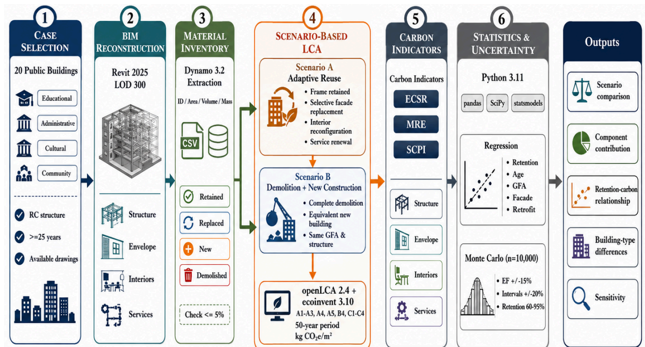
Figure 1. BIM-based life cycle assessment framework for evaluating embodied carbon reduction in adaptive reuse of existing public buildings
