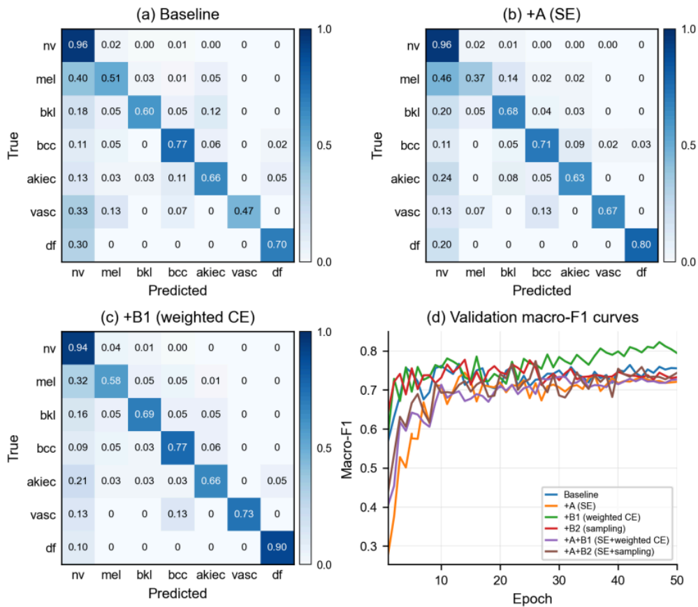
Figure 1. Ablation results: (a) Baseline, (b) +A(SE), (c) +B1(weighted CE) confusion matrices, (d) validation macro-F1 curves
