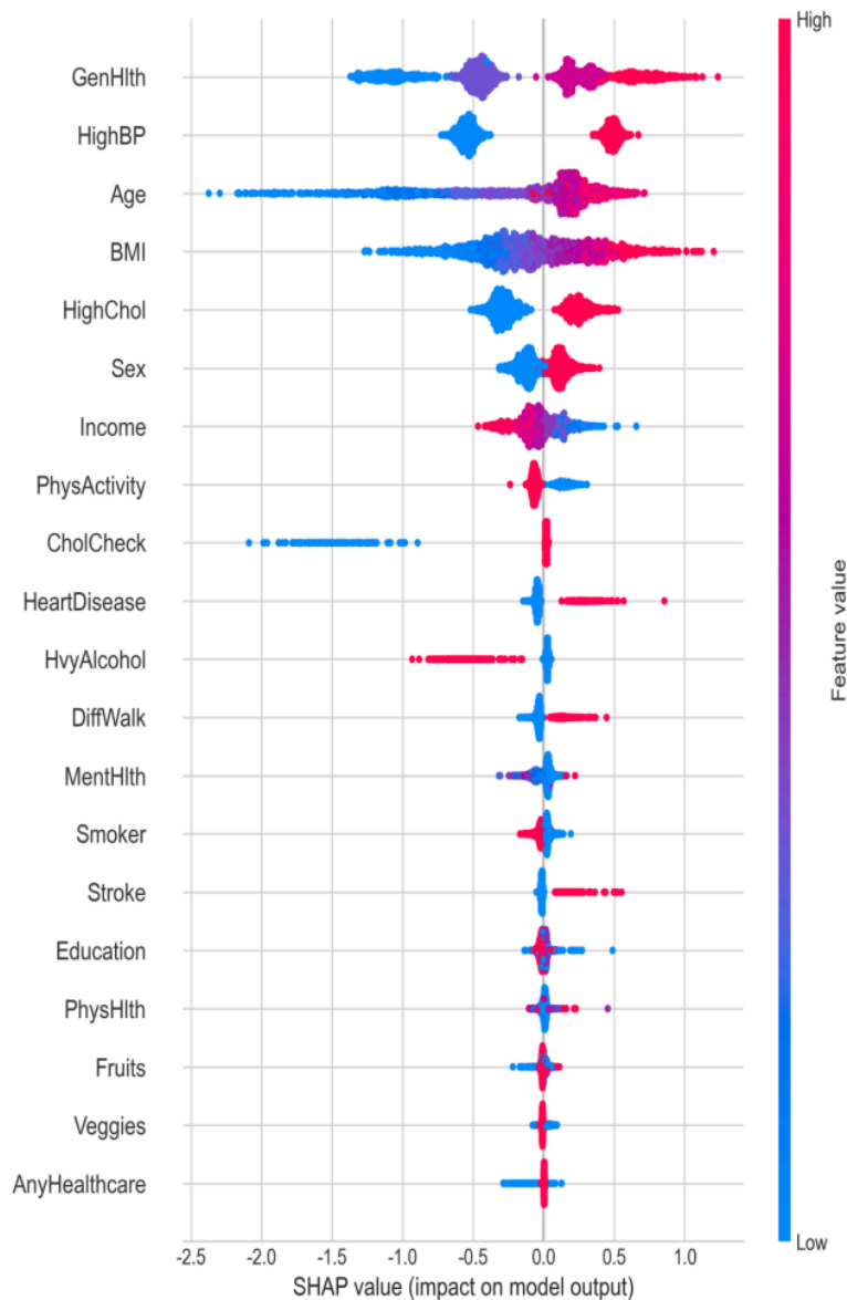
Figure 2. Summary diagram of XGBoost model SHAP (picture credit : original)
