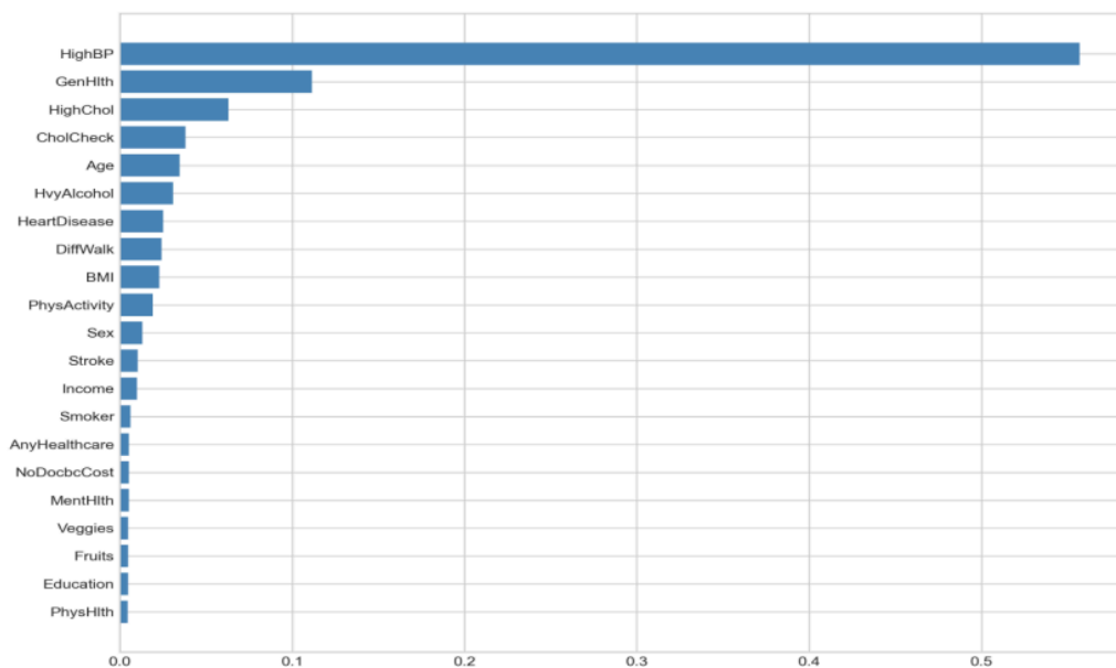
Figure 1. XGBoost feature importance feature ranking (picture credit:original)
