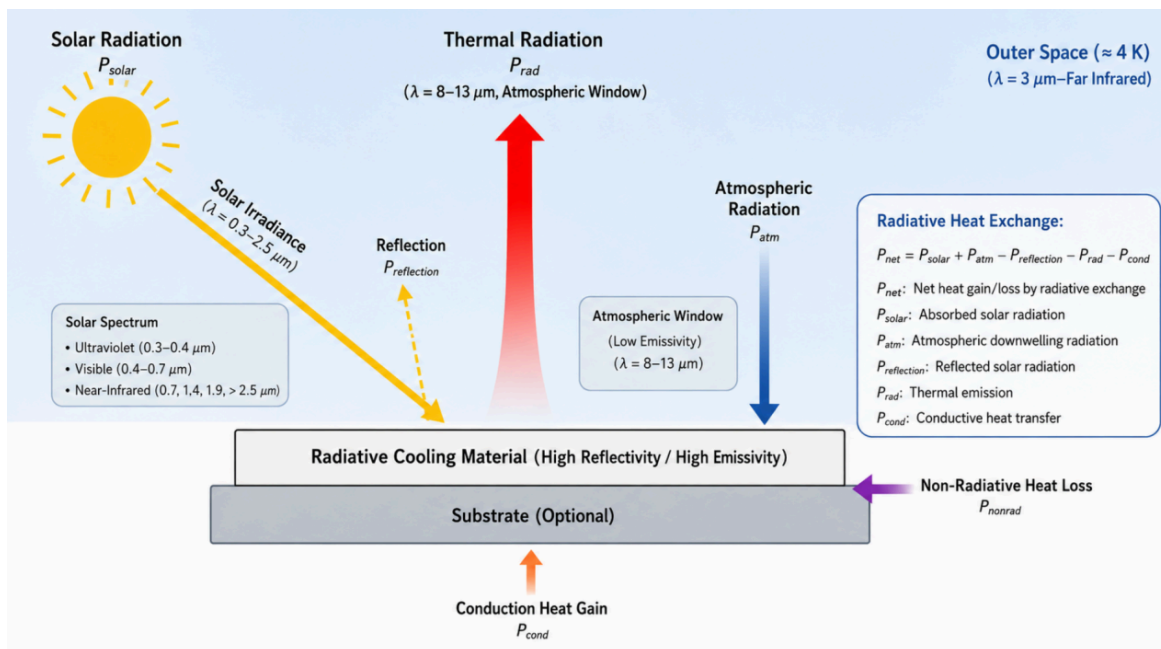
Figure 1. Energy exchange and atmospheric-window mechanism of radiative cooling
