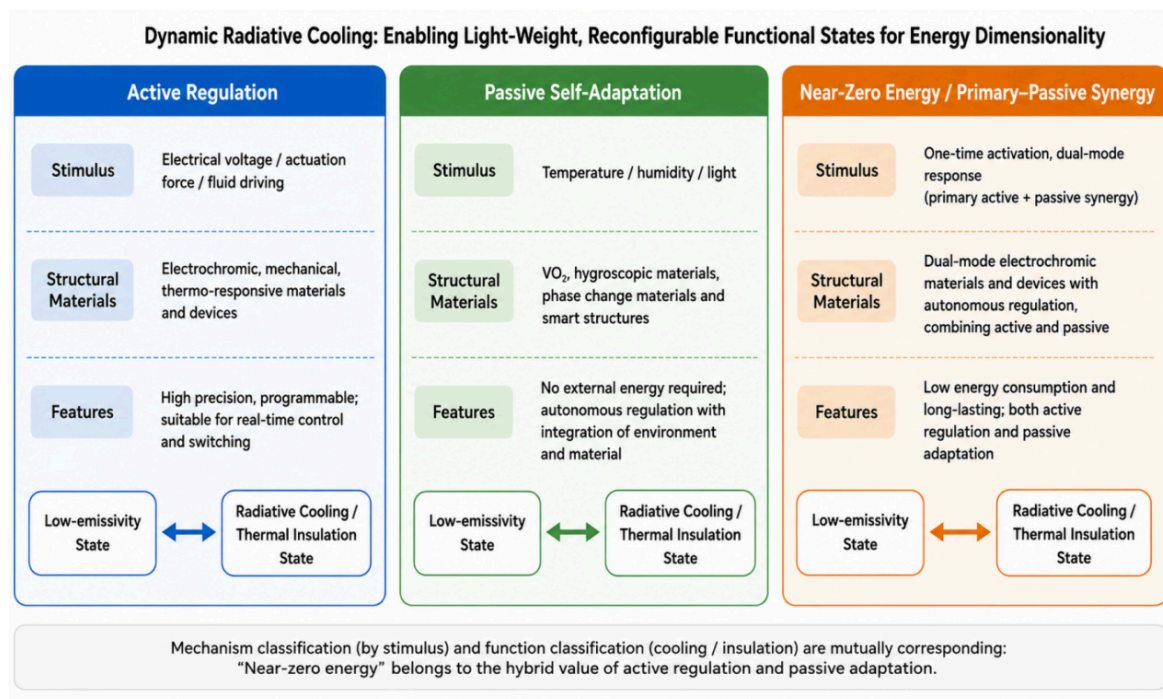
Figure 2. Regulation pathways and state switching of dynamic radiative cooling
